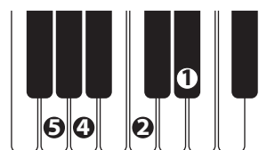
Am7b5
