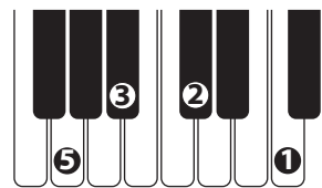
Gm7b5
