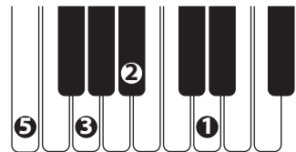
Em7b5
