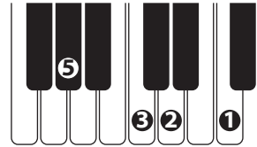
Dm7b5
