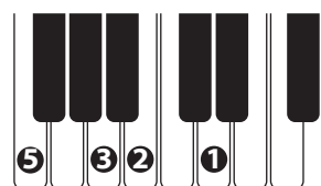
Hm7b5
