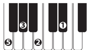
Fm7b5
